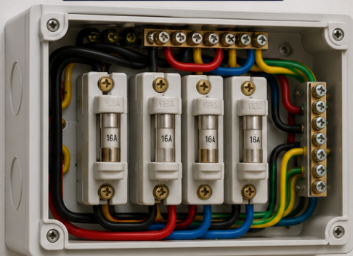
1. RE-WIREABLE FUSE BOX
