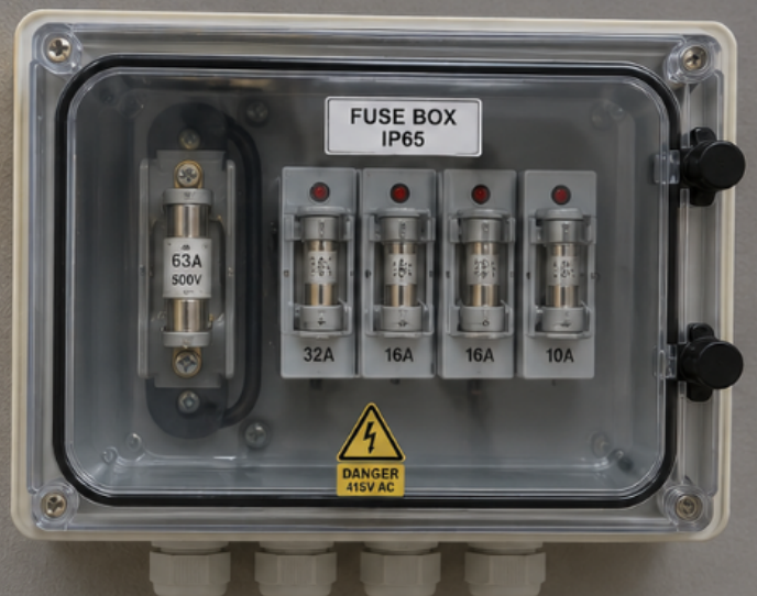
4. IP65 WEATHER PROOF FUSE BOX
