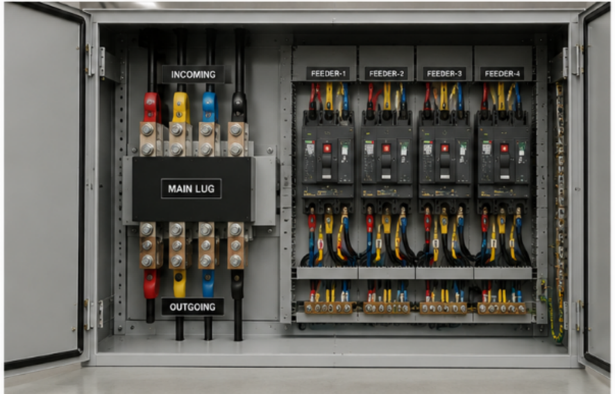
MAIN LUG PANEL – WITH OUTGOING MCCB FEEDERS
