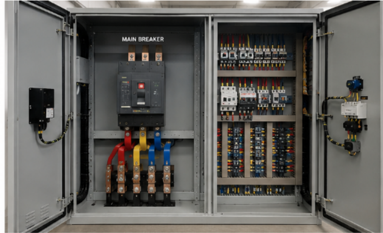
MAIN BREAKER PANEL - INTERNAL VIEW
