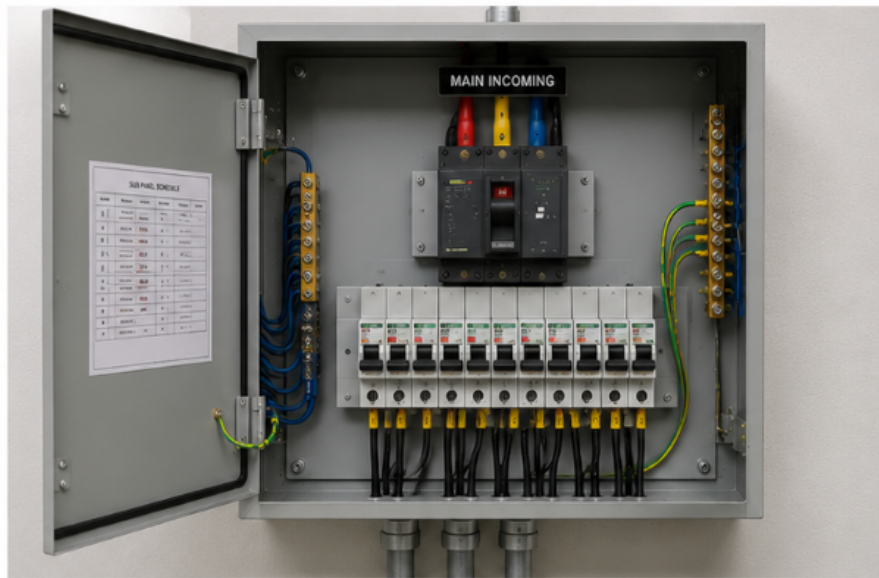
2. SUB PANEL – INTERNAL VIEW
