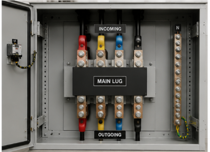
MAIN LUG PANEL – INTERNAL VIEW
